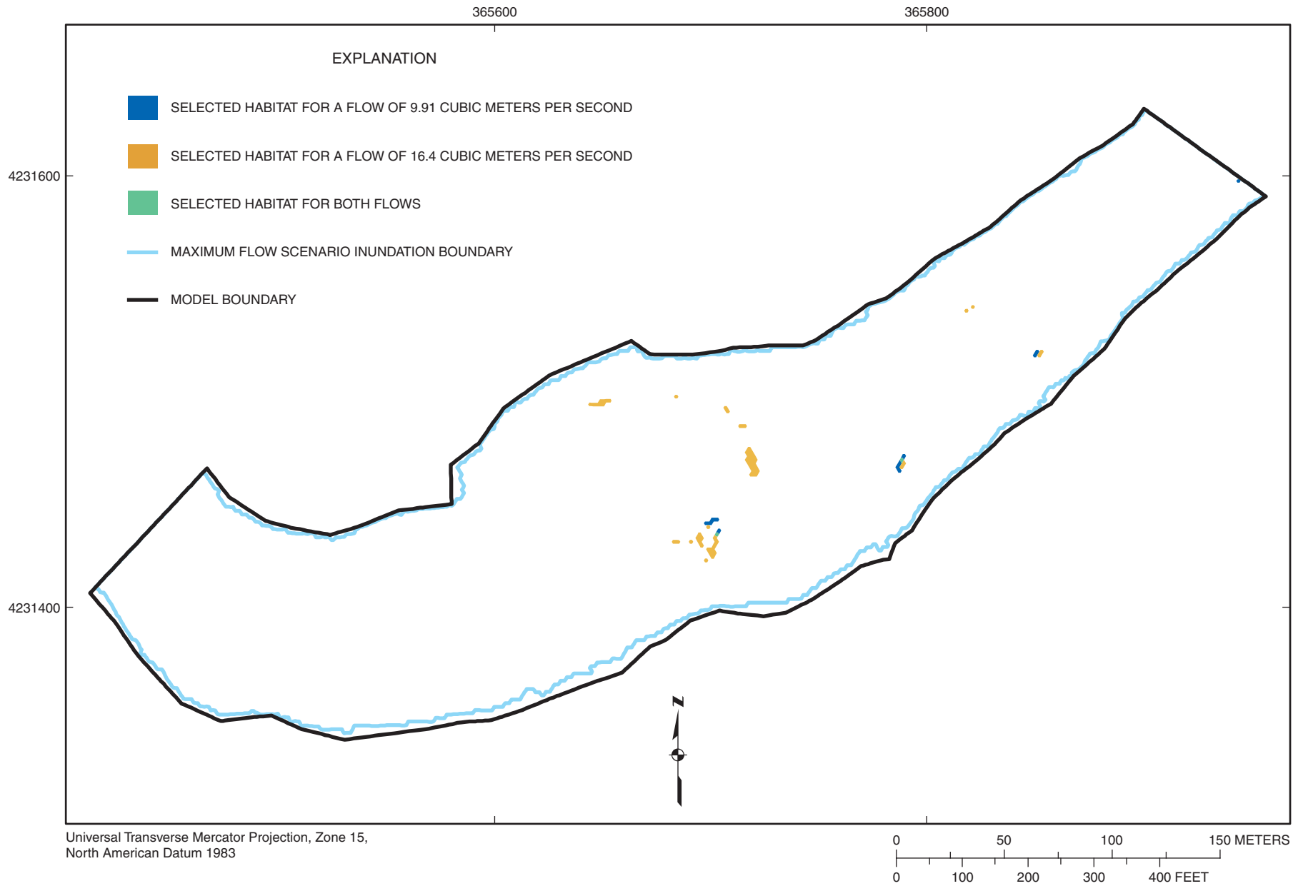
Figure 4-86. Selected habitat area distribution for habitat category 22 (channel catfish) at flows of 9.91 and 16.4 cubic meters per second at Marais des Cygnes River site MDC2.
